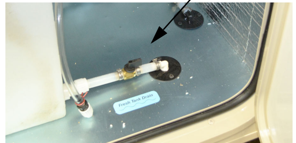
Waterline and Water Tank Drain Valves -Typical installation shown
