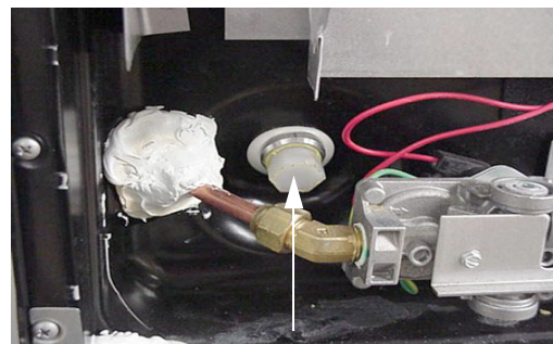
Water Heater Drain Plug (Remove with socket) -Typical View
